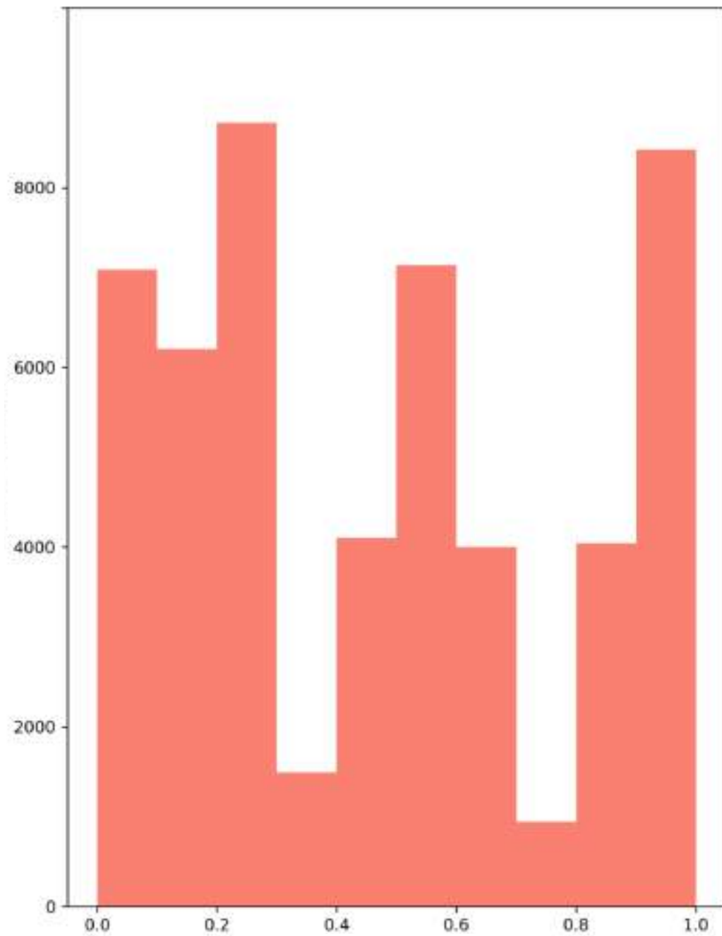
Genre scores
