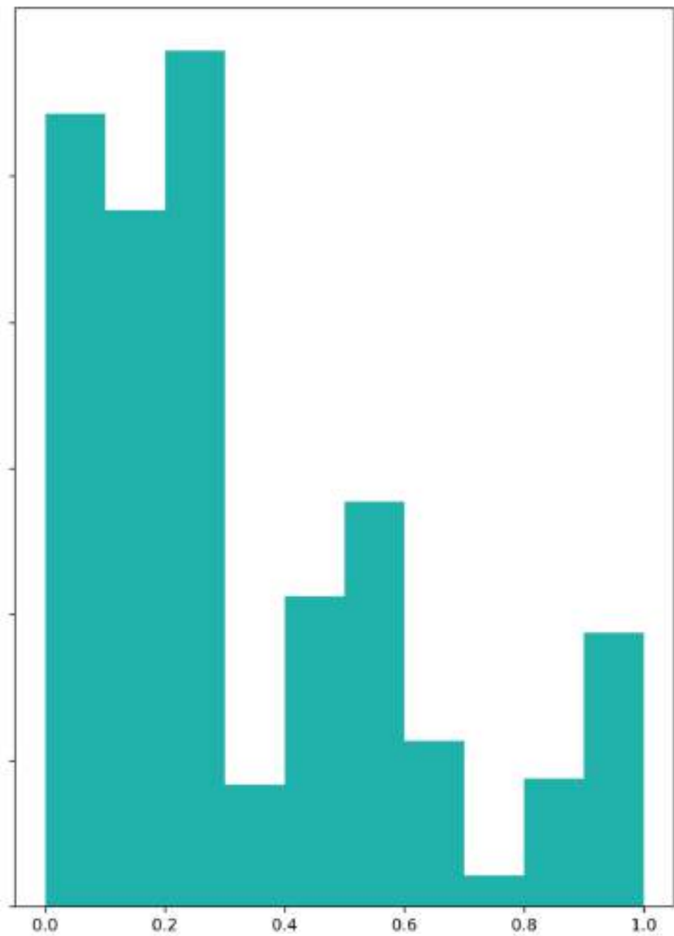
Style scores
